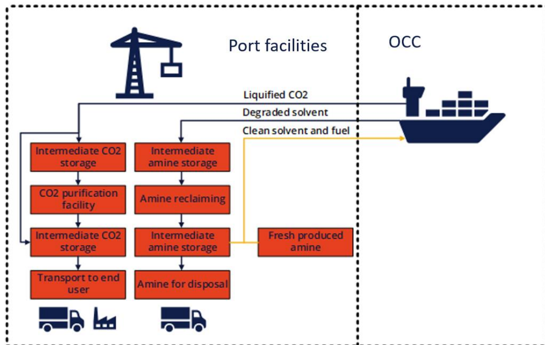
Figure 3. Infrastructure at port
