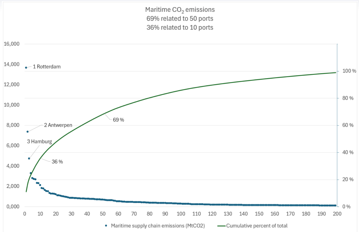
Figure 8: Plot showing the 199 Ports with total of approx. 122 Mt/year maritime CO 2 emissions (EU/EEA/UK MRV). The 50 largest covers close to 70 %. Plot based on Error! Reference source not found.
